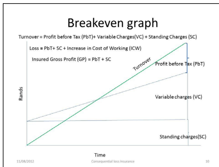
Figure 1: Breakeven graph
